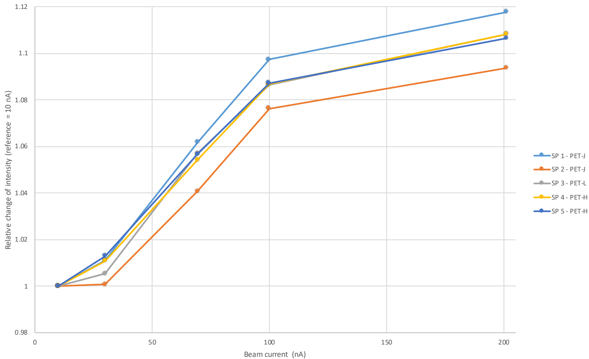
Relative change in intensity (Ti Ka in Arenal Hbl on PET monochromators)
